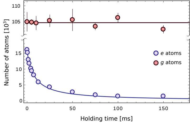
Figure 6.13: Experimental characterization of the loss rates associated to inelastic e - e collisions. Number of e atoms (in blue) and g atoms (in red) as a function of the holding time in the lattice after a clock excitation pulse in a 1D lattice. The red line represents the mean value of g atoms, while the blue line is the result of a fit to the e data with the model in equation (6.23), assuming the scaling in equation (6.30).
