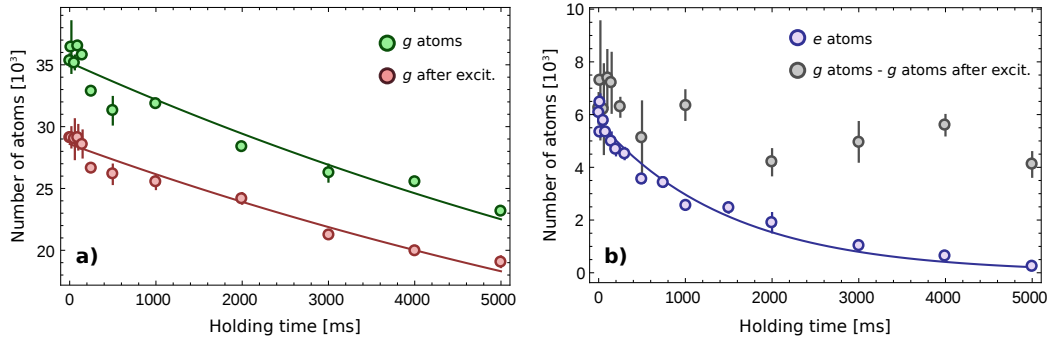
Figure 6.12: Experimental characterization of the loss rates associated to inelastic e - g collisions. Inelastic e - g collisions have been investigated by exciting atoms from the |gg\rangle state to the |eg\rangle state by selectively addressing the |gg\rangle \rightarrow |eg\rangle transition in a 3D optical lattice ( s = 27.5 ). a: The number of atoms remaining in g after the clock pulse (red) is compared with the number of atoms in the absence of clock excitation (green) as a function of the holding time in the lattice (the slow decay of both datasets shows the finite single-particle lifetime in the lattice). Lines are exponential fits of the experimental data that must be intended as guides to the eye. b: The number of atoms detected in the e state (blue) is shown as a function of the holding time in the lattice after the excitation of the transition. This number is compared with the difference between the number of g atoms without and with the clock excitation (gray), which displays an approximately time-independent behavior. The solid blue line is an exponential fit of the experimental data.
