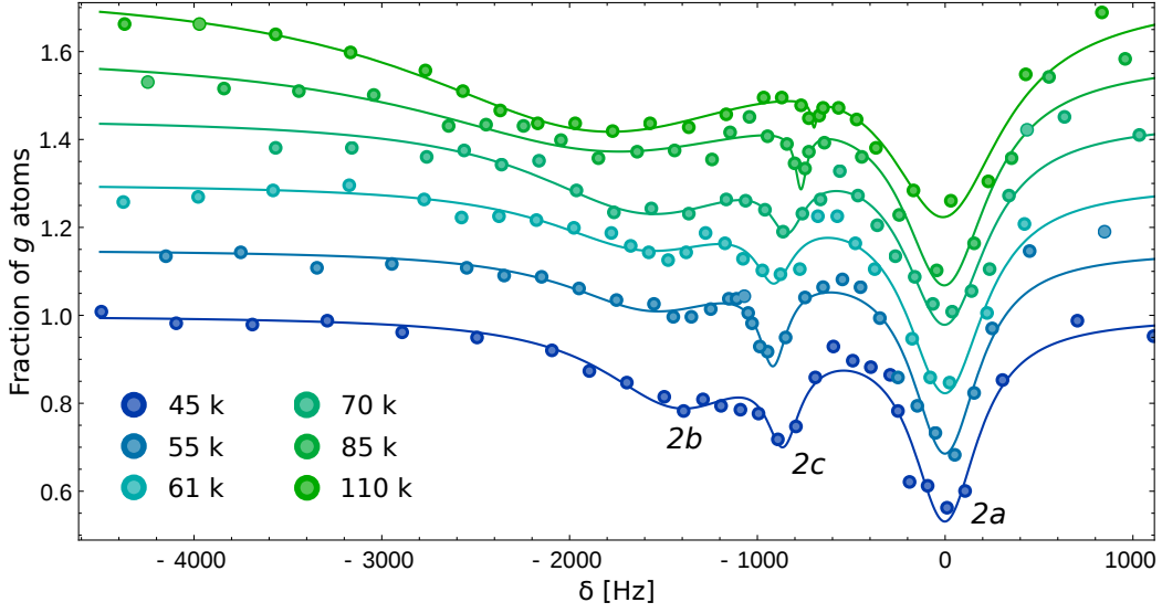
Figure 6.8: Clock spectroscopy as a function of the atom number performed in an anisotropic 3D lattice characterized by the depths s_{x,y,z} = \{15, 30, 15\} . An additional peak (labelled as 2c) is revealed between the peaks 2b and the blue sideband (2a) as the atom number is reduced (see the main text for details). Frequency offsets are given with respect to the peak 2a.
