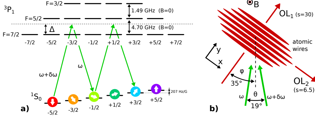
Figure 5.1: a: Scheme of the Yb levels involved in the Raman transitions. The value of the Raman detuning is \Delta = 1.876 GHz. b: Sketch of the experimental setup showing the relative position of the Raman beams (in green) with respect to the optical lattices and the one dimensional fermionic tubes (in red).
