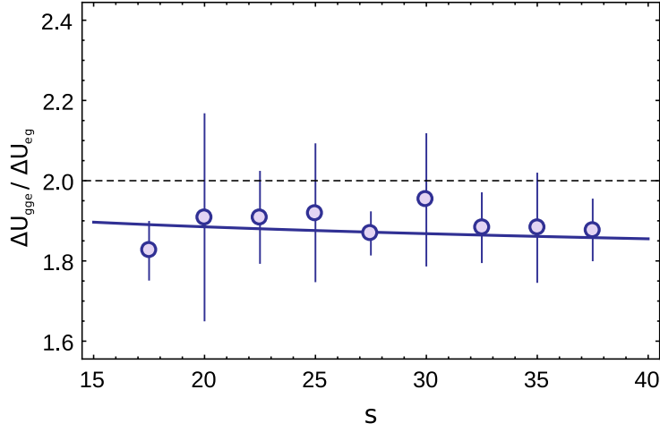
Figure 6.5: Ratio between the energy shift relative to the three-particles peak ( |ggg\rangle \rightarrow |gge\rangle transition) and the one relative to the two-particles peak ( |gg\rangle \rightarrow |ge\rangle transition). The line is the theoretical prediction evaluated using the equation 6.15.
