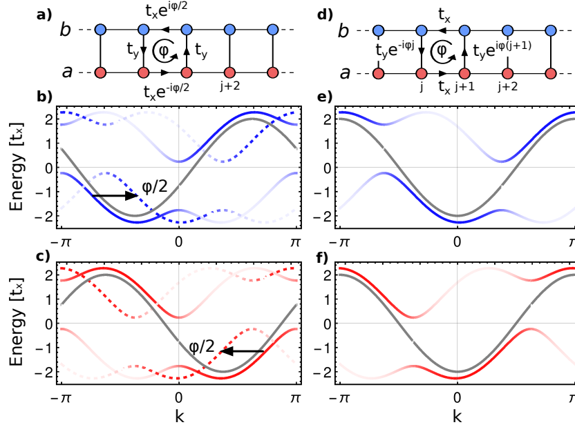
Figure 2.5: Two-leg ladders. Sketch of a two-leg ladder pierced by a uniform magnetic flux in the "unphysical" gauge (a) (complex tunnelling along the long dimension) and in the "physical" gauge (d) (complex tunnelling along the short dimension). b-c spectra in the "unphysical" gauge of the upper leg (b) and of the lower leg (c) for the flux \Phi = 0.75\pi : solid blue-red lines for t_x = t_y , dotted blue-red lines are the same spectra in the "physical" gauge", gray lines for t_y = 0 . e-f spectra in the "physical" gauge of the upper leg (e) and of the lower leg (f) for the flux \Phi = 0.75\pi : solid blue-red lines for t_x = t_y , gray lines for t_y = 0 . In b-c-e-f the intensity of the colors reflects the squared module of the wavefunction.
